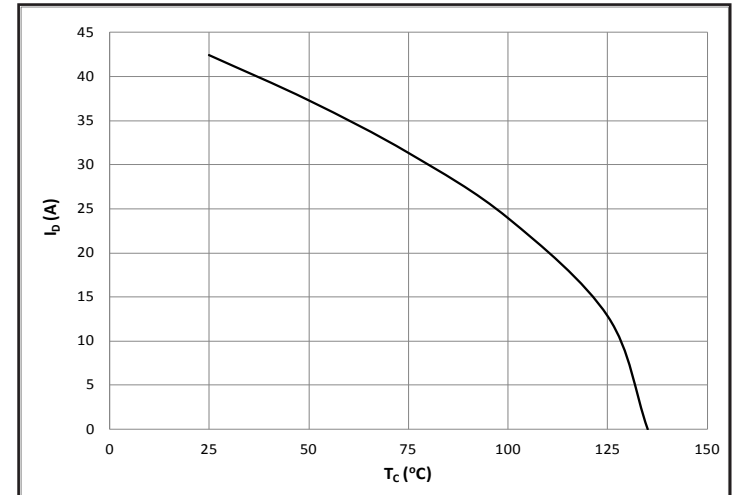
Figure 10. Continuous Current Derating Curve
