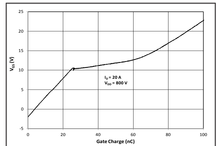
Figure 12. Typical Gate Charge Characteristics (25°C)
