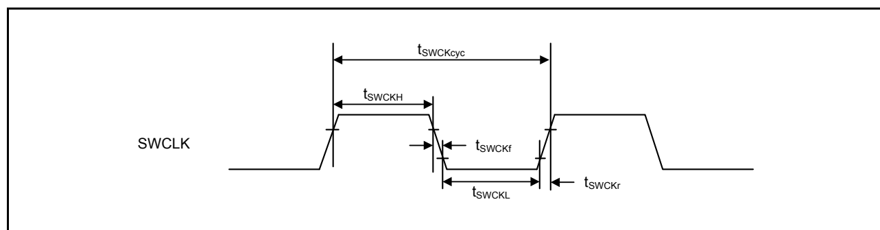
Figure 2.99 SWD SWCLK timing
