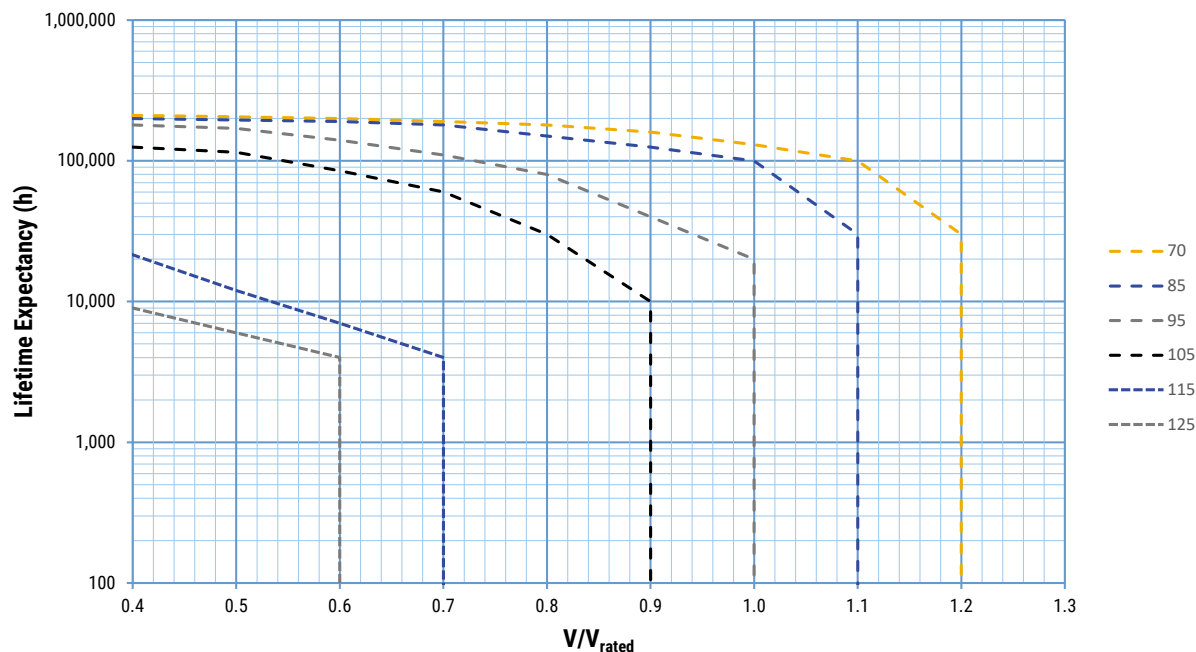
Lifetime Curve at Hot Spot Temperature
